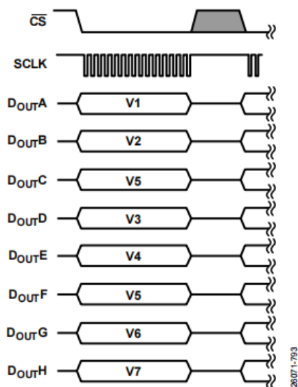
Figure 106. Serial Interface ADC Reading, Eight DOUTX Lines
