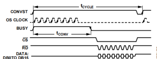
Figure 87. AD7606C-16 Oversampling by 8 Example, Read After Conversion, Parallel Interface, OS_CLOCK is the Internally Generated Sampling Signal
