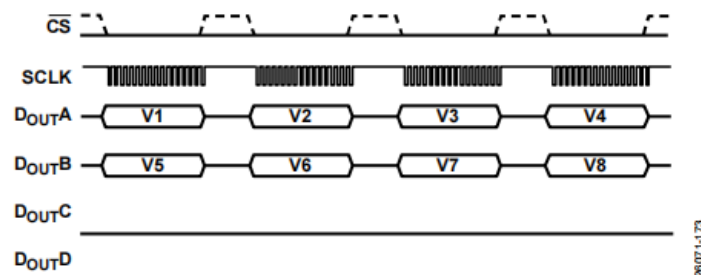
Figure 104. Serial Interface ADC Reading, Two D OUT x Lines
