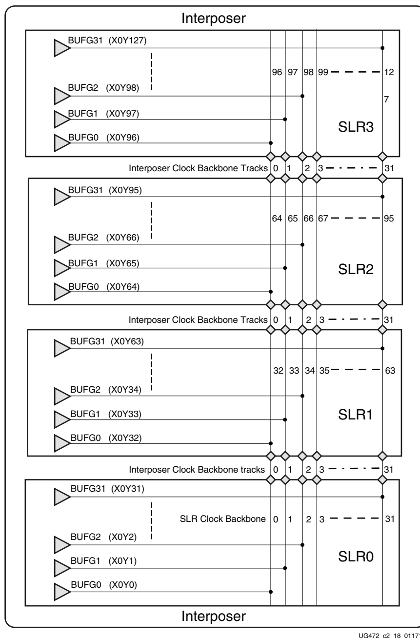
Figure 2-30: BUFG Connectivity across Interposer Clock Backbone
