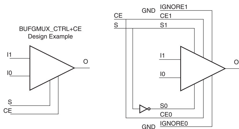
Figure 2-17: BUFGMUX_CTRL with a CE and BUFGCTRL
