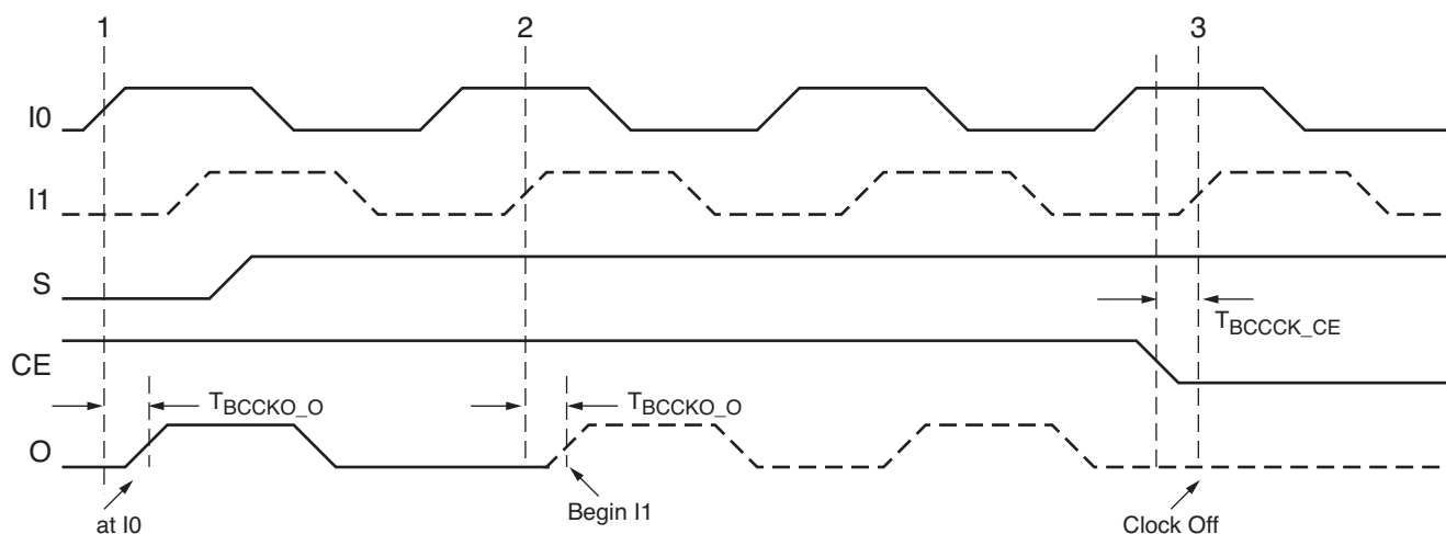
Figure 2-18: BUFGMUX_CTRL with a CE Timing Diagram
