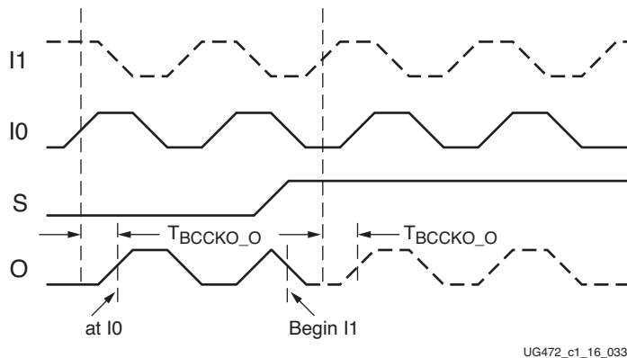
Figure 2-16: Asynchronous MUX Timing Diagram
