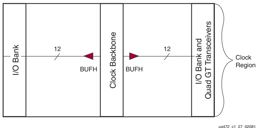
Figure 2-27: Example of a Horizontal Clock Buffer
