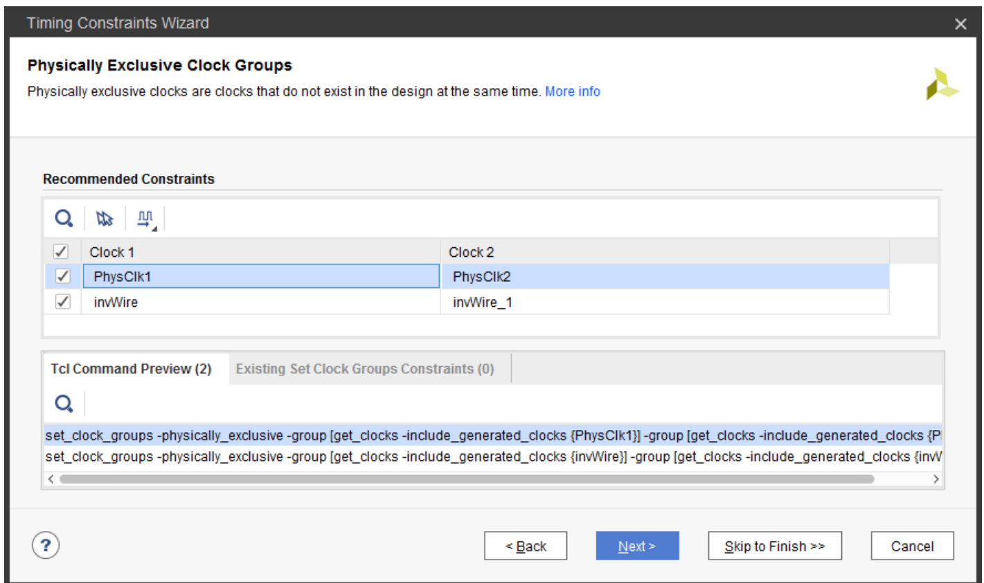
Figure 26: Example of a Design with Clock Groups Constraint
