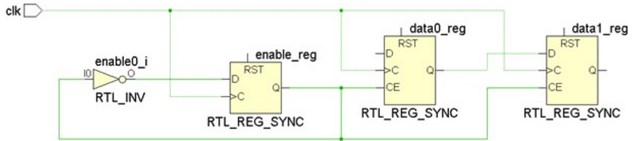
Figure 61: Registers Enabled Every Two Cycles
