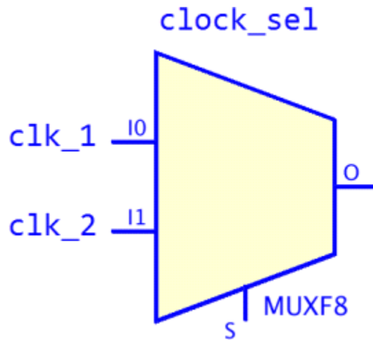
Figure 89: Clock Example
