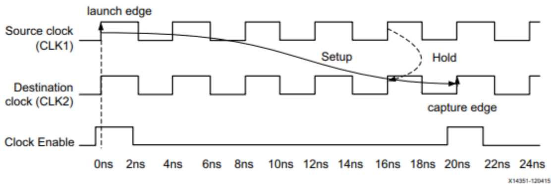
Figure 66: Setup=5, Hold=4
