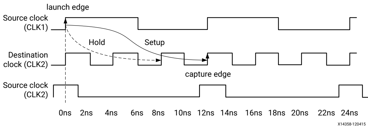
Figure 75: Setup=3, Hold Moved Accordingly
