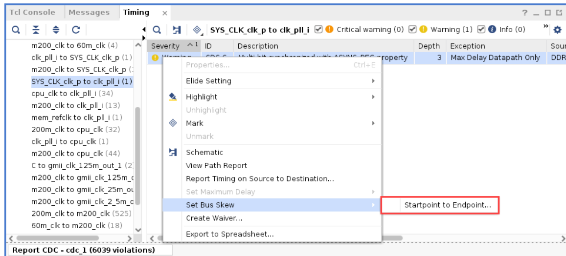
Figure 93: Setting Bus Skew within Report CDC
