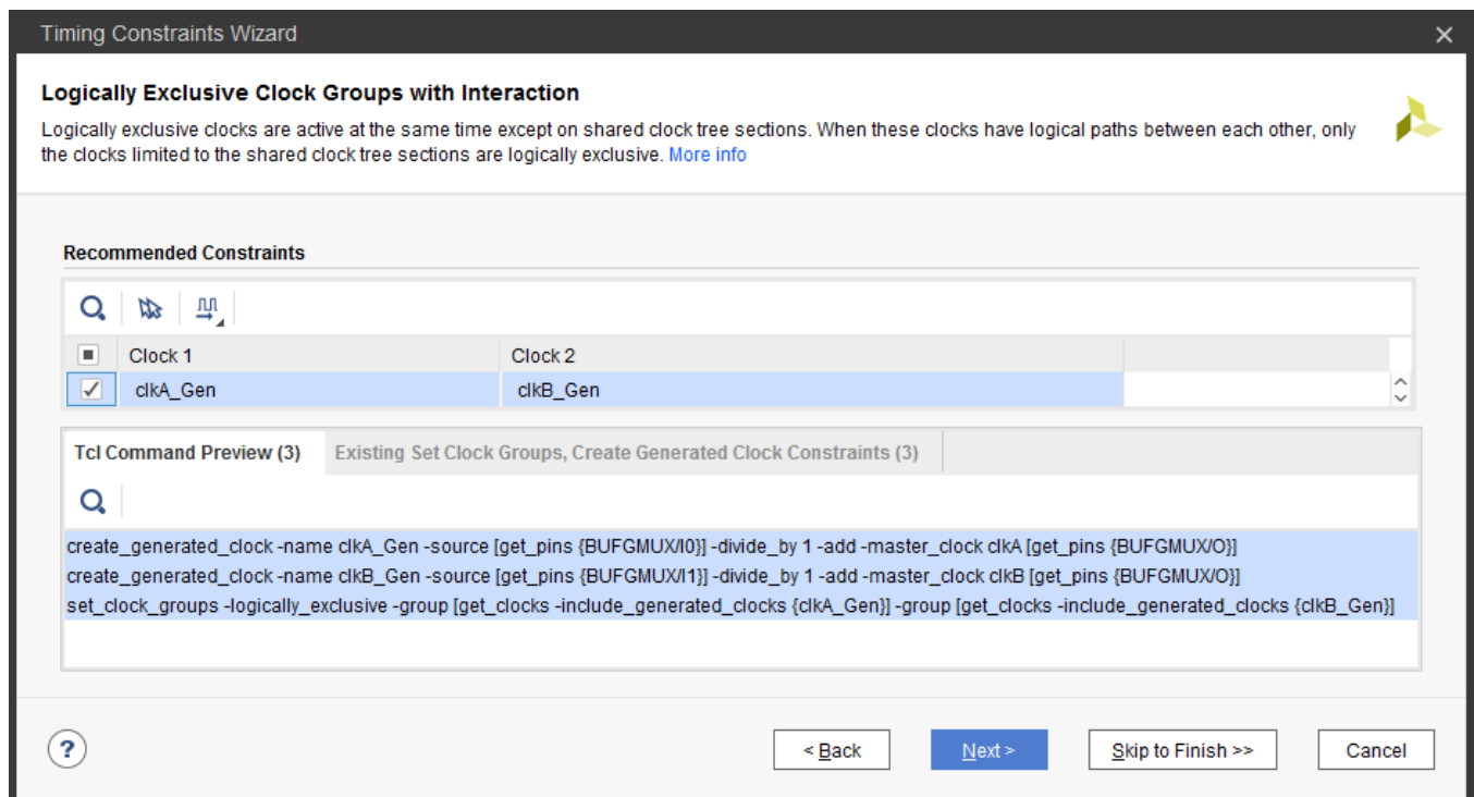
Figure 29: Recommended Constraints for Logically Exclusive Clocks with Interaction
