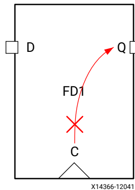
Figure 85: Timing Not Propagating after Path Segmentation
