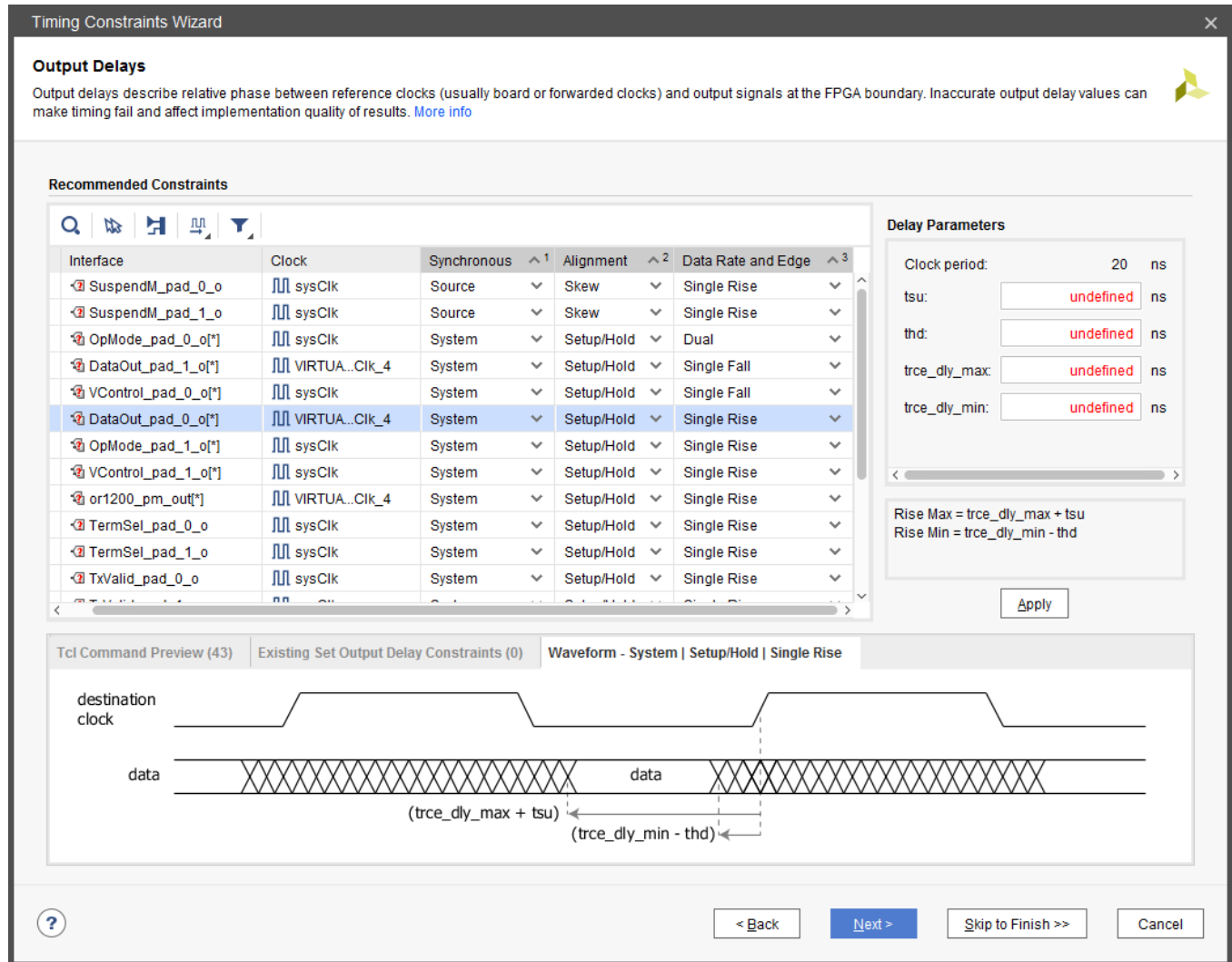
Figure 20: Recommended Output Delay Constraint Templates
