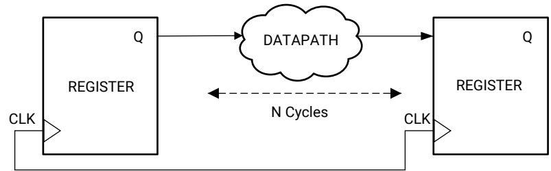
Figure 59: Multicycle Constraint in Single Clock Domain
