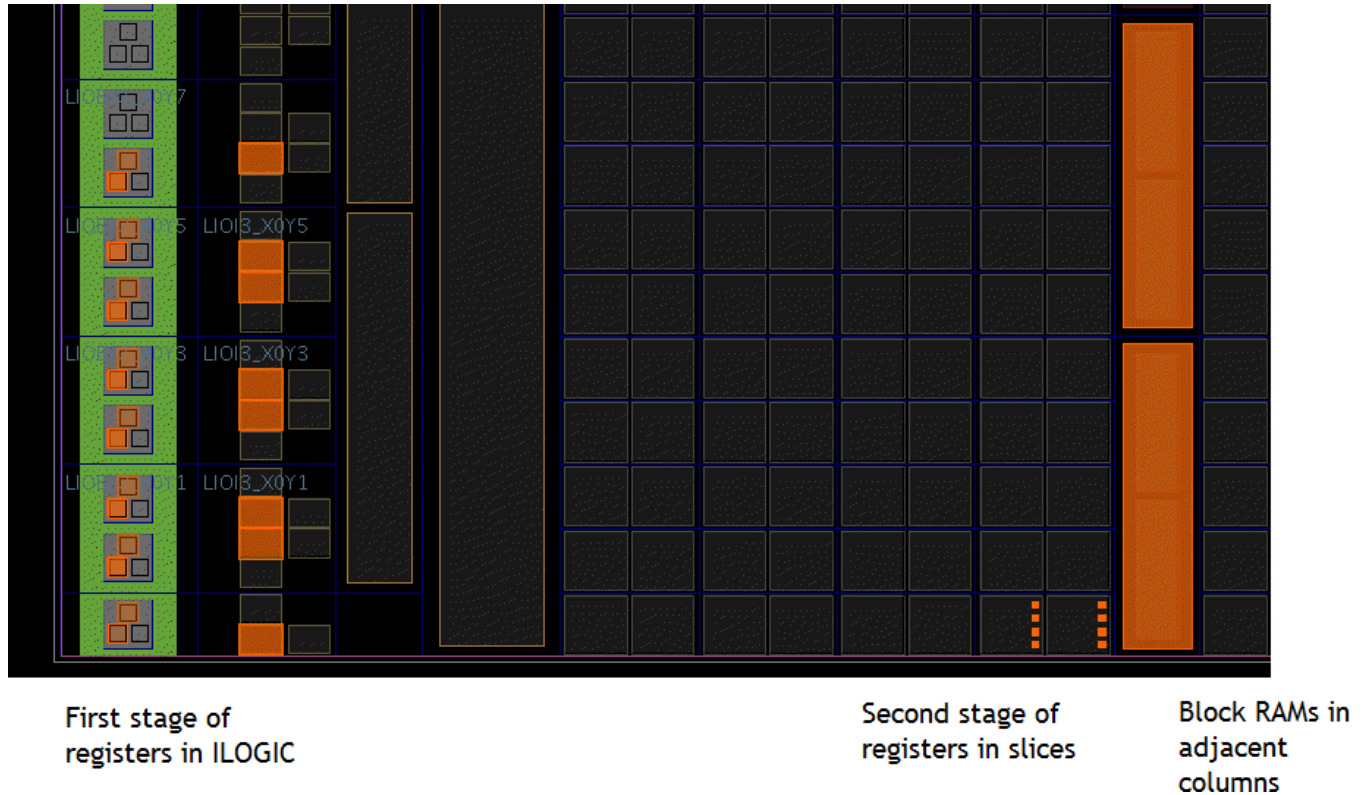
Figure 101: Manually Placed Cells for an Absolute Grid Macro
