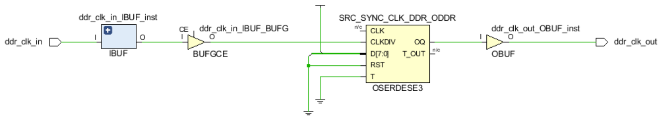
Figure 15: UltraScale Forwarded Clock Typical Circuitry
