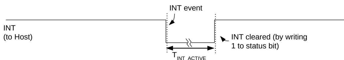
Figure 6. INT Pulse on Event other than HTPLG
